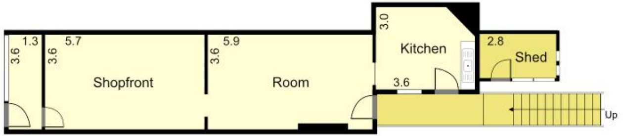
Ground Floor
