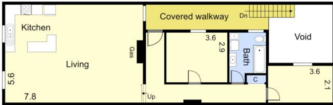
First Floor
