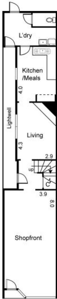
GROUND FLOOR
