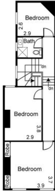
FIRST FLOOR
