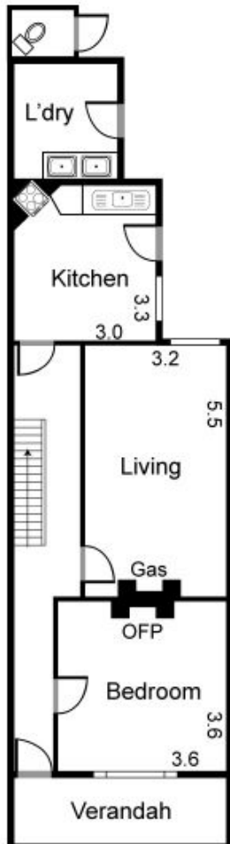
Ground Floor
